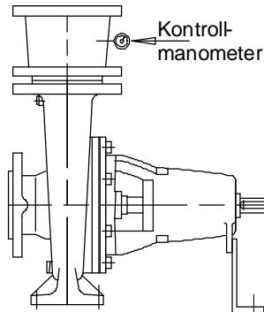
Kontrollmanometerinstallation
