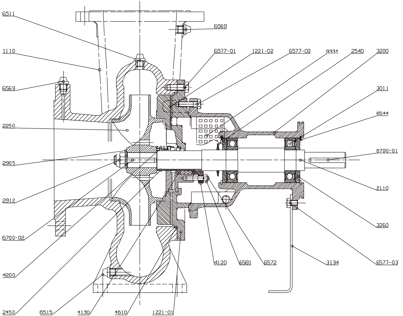
Pumpe ME Lager 32/42
